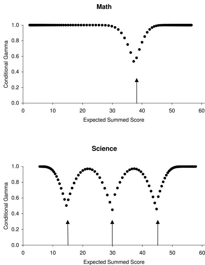
Figure 2: Estimates of \gamma_\theta
